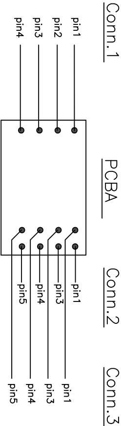
Pin Assignment
