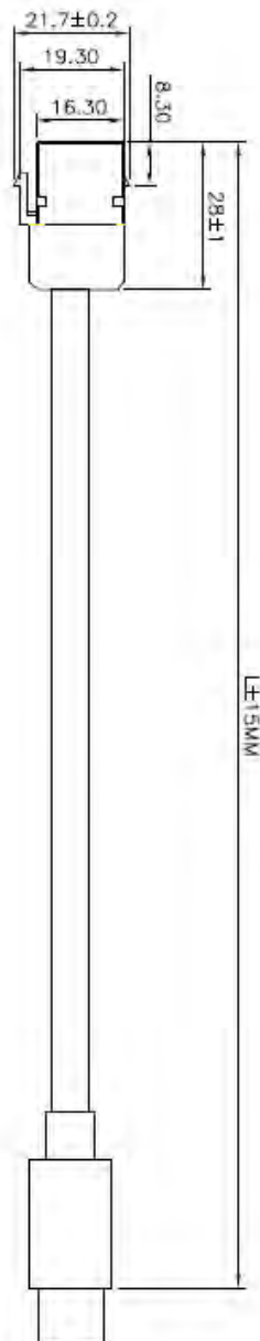
P1 USB3.1 Type-C Female
