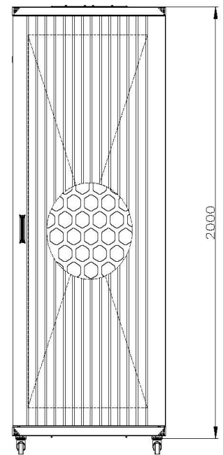
BACK (Metal Door fully perforated)
