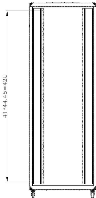
Without front door
