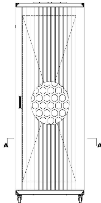
FRONT (Metal Door fully perforated)
